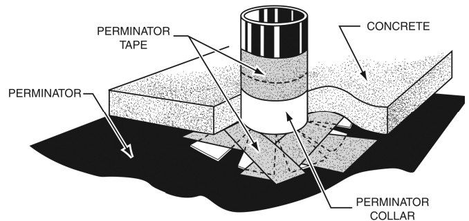
Figure 2: COLLAR INSTALLATION
